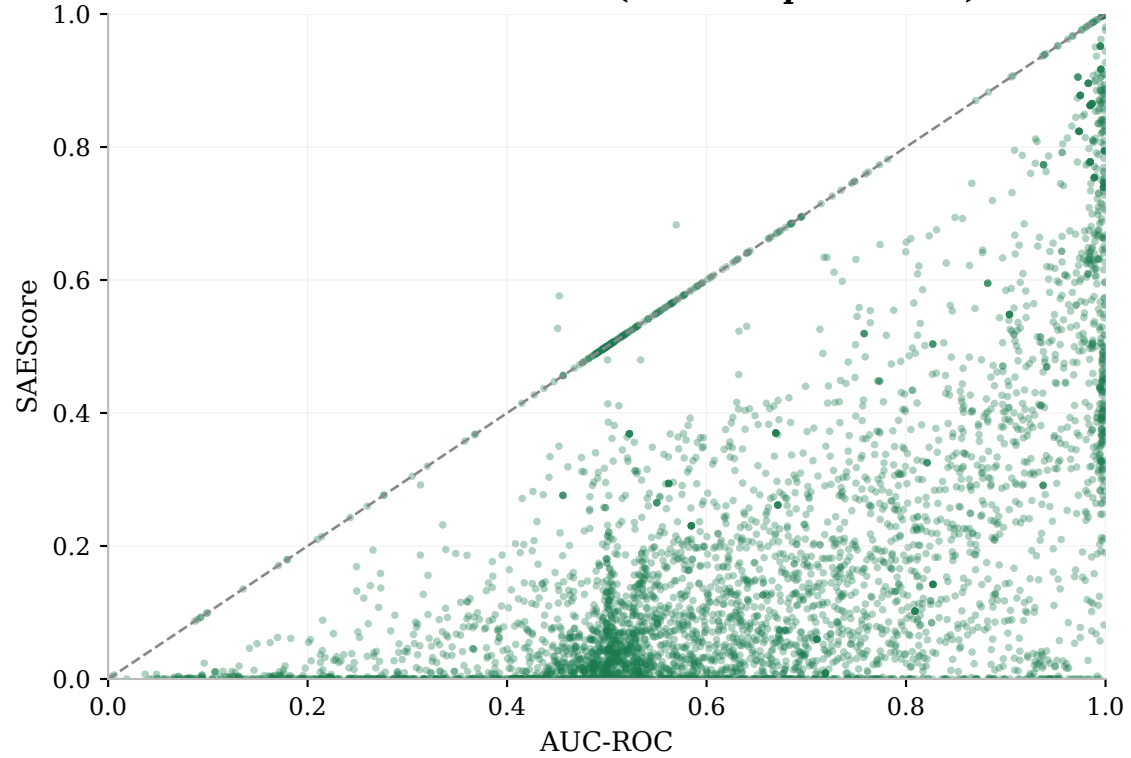
(b) AUC-ROC vs SAEScore (all recomputed rows)
